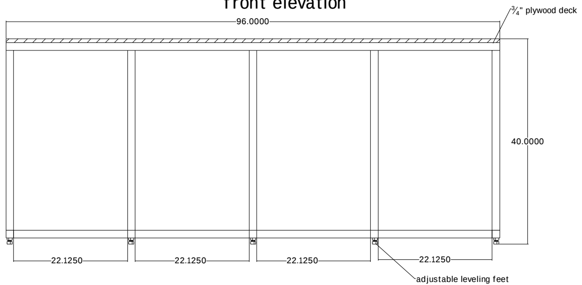
front elevation
